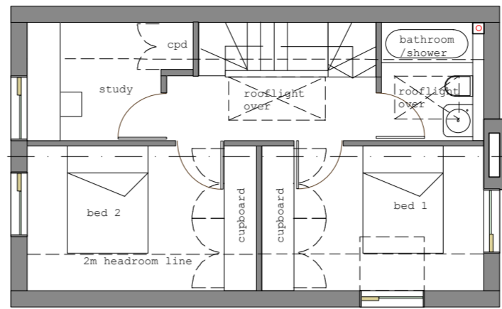
House 2 First Floor Plan 1.100
