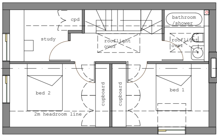
House 1 First Floor Plan 1.100
