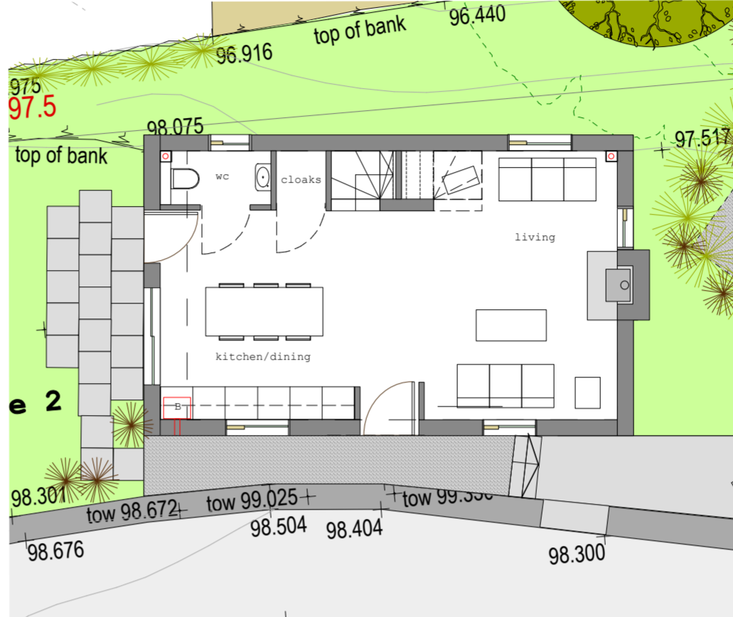
House 2 Ground Floor Plan 1.100
